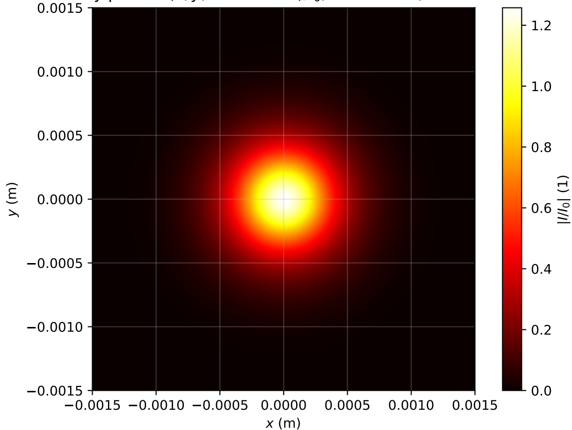
Intensity profile I(x, y, z = 0.876m)/I_0 , P_{in}=0.8P_{cr} , artificial time
